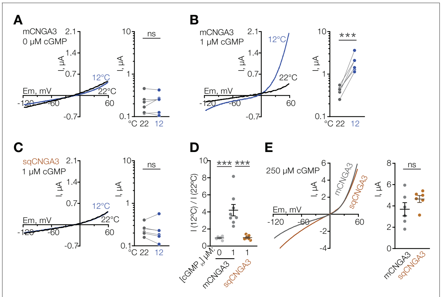
Figure 4. Cooling potentiates mouse but not squirrel CNGA3 in oocytes. (A–C) Exemplar whole-cell currents (left) and quantification of current amplitude at 60 mV (right) recorded in Xenopus oocytes expressing mouse or squirrel CNGA3 in response to a voltage ramp in the presence or absence of 1 \mu\text{M} intracellular cGMP. (D) Quantification of the magnitude of cold activation of CNGA3 current in oocytes at 60 mV in the presence of 1 \mu\text{M} intracellular cGMP. (E) Exemplar whole-cell current traces (left) and quantification of current amplitude at 60 mV (right) recorded from mouse or squirrel CNGA3 in response to a voltage ramp in the presence of saturating 250 \mu\text{M} intracellular cGMP. Data are mean \pm SEM. NS, not significant, p > 0.05 ; *** p < 0.001 , paired t-test (A–C), Dunnett's test (D), t-test (E). Each dot represents an individual cell.
