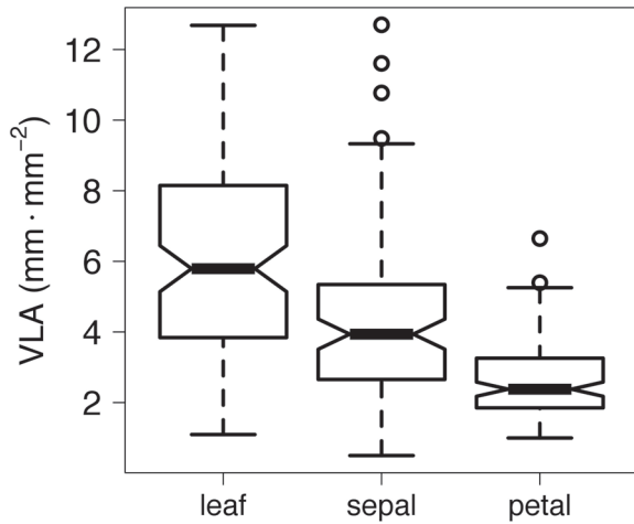
Fig. 1. Boxplot of VLA for leaves, sepals, and petals. All pairwise differences are highly significant ( P < 0.001 ). Median values are indicated by the solid line in the middle of the boxes.
