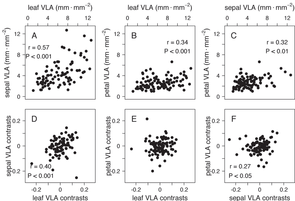
Fig. 3. Pairwise (A–C) trait and (D–F) phylogenetic independent contrast correlations. Correlation coefficients and P values are shown for statistically significant correlations based on Spearman rank tests.
