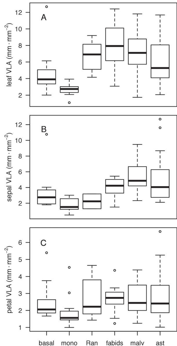
Fig. 2. Boxplots of VLA for (A) leaves, (B) sepals, and (C) petals for each major clade included in this study. Basal, magnoliids and Austrobaileyales; mono, monocots; Ran, Ranunculales; malv, malvids; ast, asterids. See Supplementary Table S1 for list of species in each clade.
